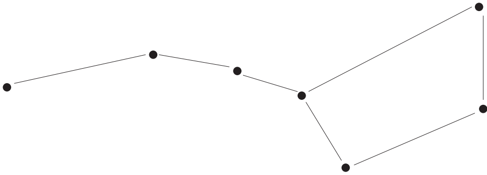
Ursa Major
